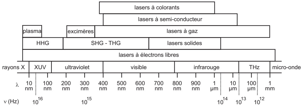
Figure 3 - Couverture spectrale des lasers.
